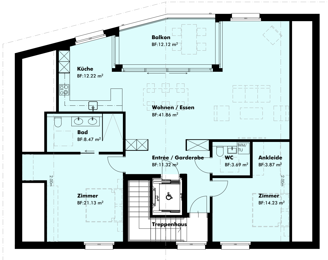
WHG 12-04-01 3.5 Zimmer
